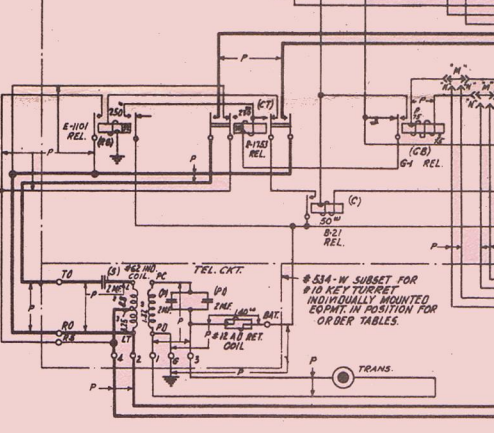
FIG. 4 OPERATOR'S TRIPPING & TELEPHONE CKTS.
