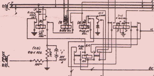
FIG. 7 NON-LOCKING INTERCEPTING LINE CKT. (SEE NOTE 7)
