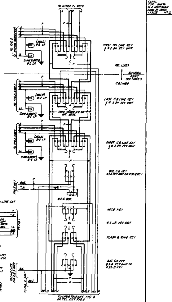
FIG. 7 OPERATOR'S TELEPHONE CXT (SEE NOTE 7)
