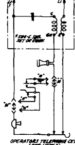
FIG. 7 OPERATOR'S TELEPHONE CXT (SEE NOTE 7)
