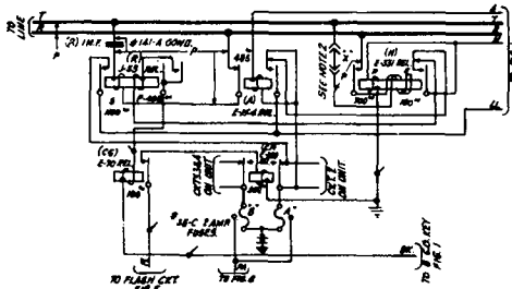
FIG. 3 INTERCEPTING LINE CXT.
